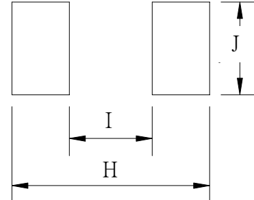
LAND PATTERNS(mm)
